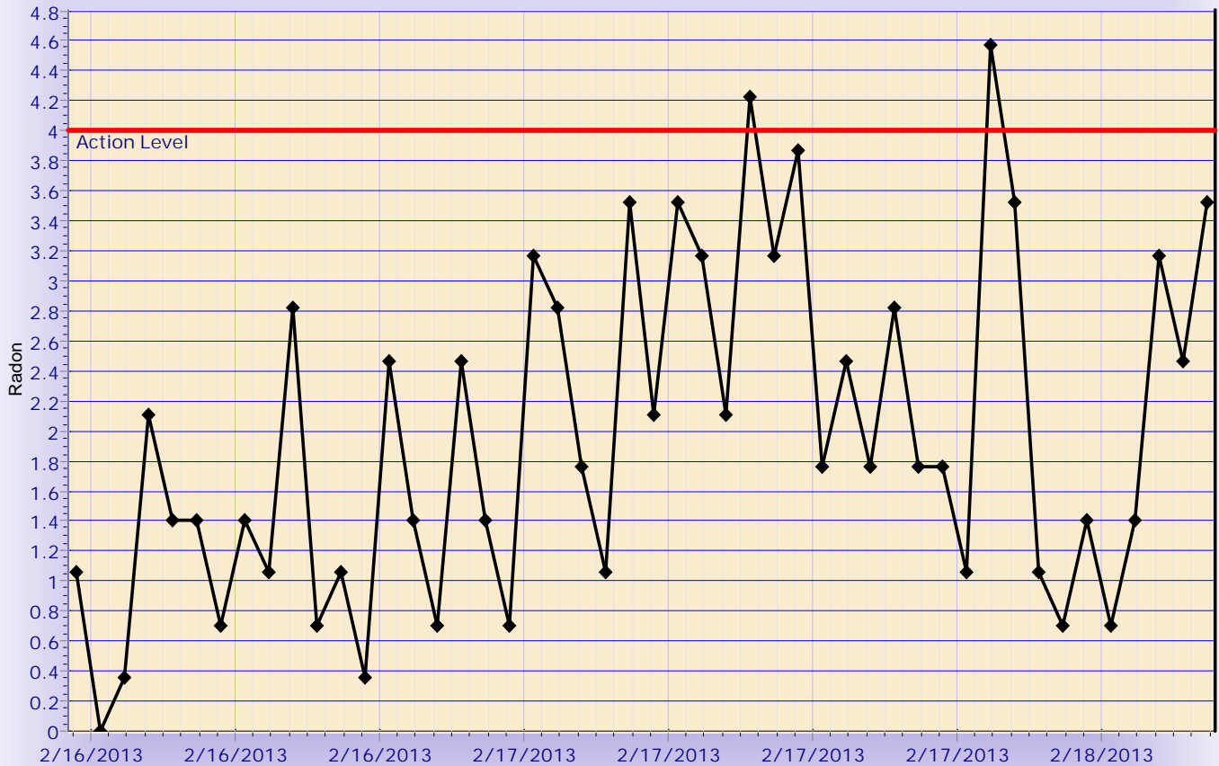
Continuous Radon Monitor
